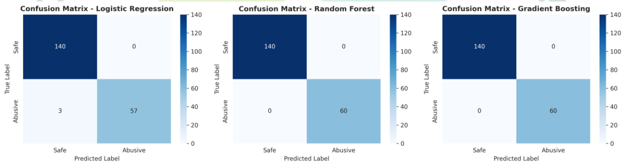
Figure 3: Confusion Matrices for Classification Models
